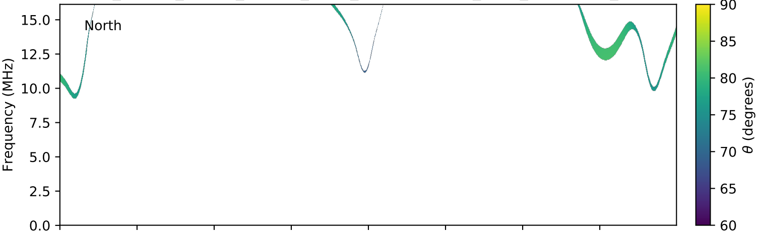
expres_cassini_jupiter_europa_isaac_lossc-wid1deg_3kev_20011028_v01.cdf
