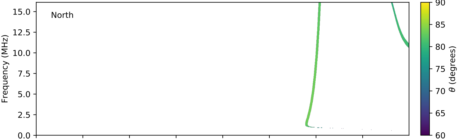
expres_cassini_jupiter_europa_isaac_lossc-wid1deg_3kev_20011027_v01.cdf
