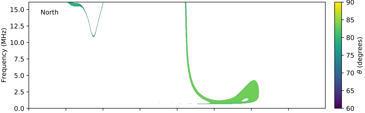
expres_cassini_jupiter_europa_isaac_lossc-wid1deg_3kev_20011025_v01.cdf
