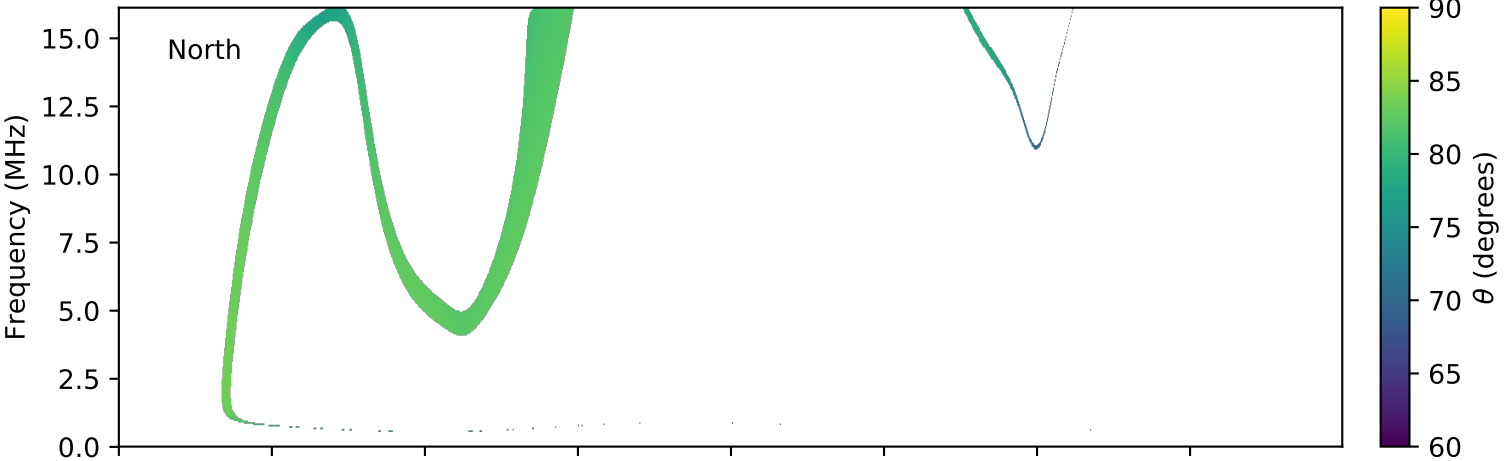
expres_cassini_jupiter_europa_isaac_lossc-wid1deg_3kev_20011024_v01.cdf
