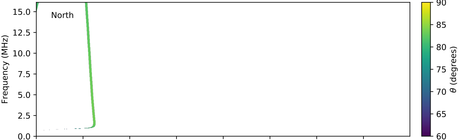
expres_cassini_jupiter_europa_isaac_lossc-wid1deg_3kev_20011022_v01.cdf
