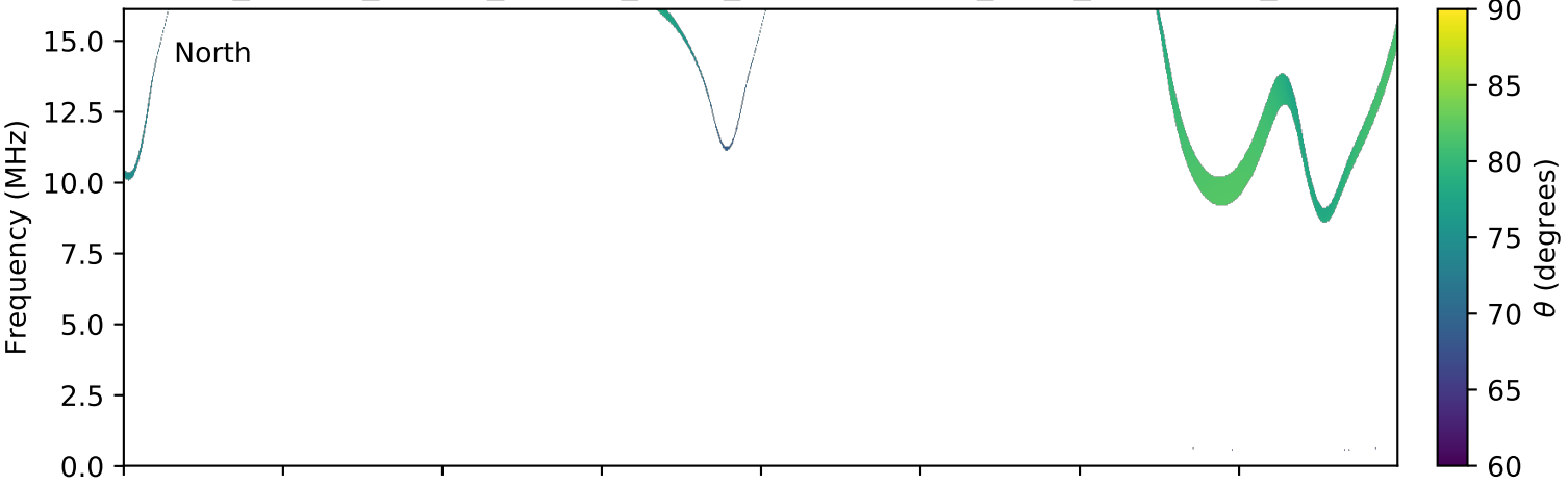
expres_cassini_jupiter_europa_isaac_lossc-wid1deg_3kev_20011021_v01.cdf
