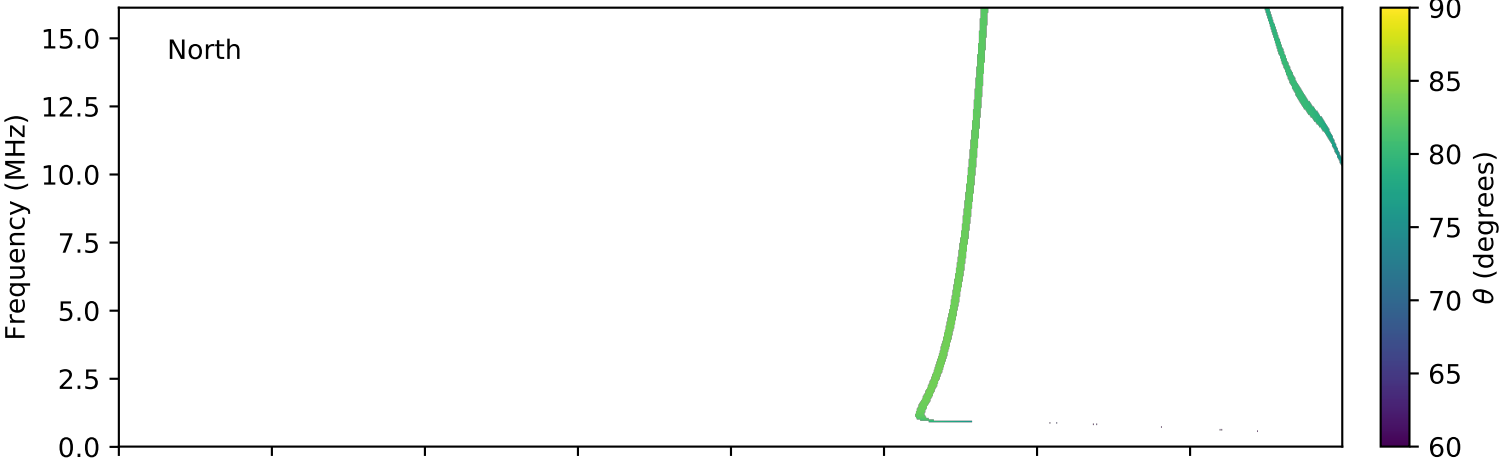
expres_cassini_jupiter_europa_isaac_lossc-wid1deg_3kev_20011020_v01.cdf
