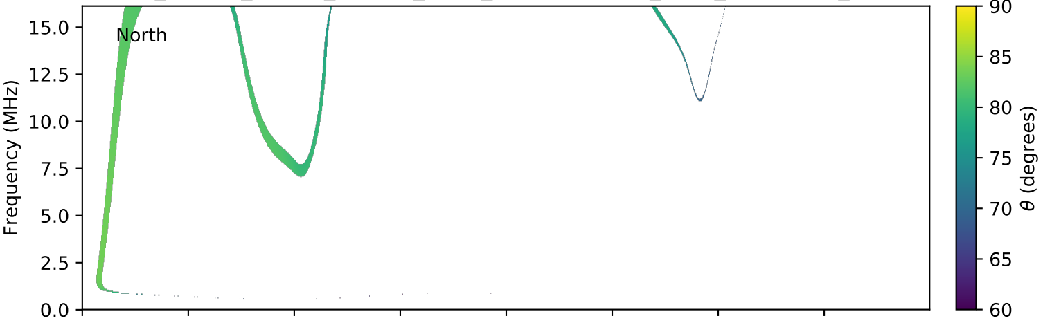
expres_cassini_jupiter_europa_isaac_lossc-wid1deg_3kev_20011017_v01.cdf
