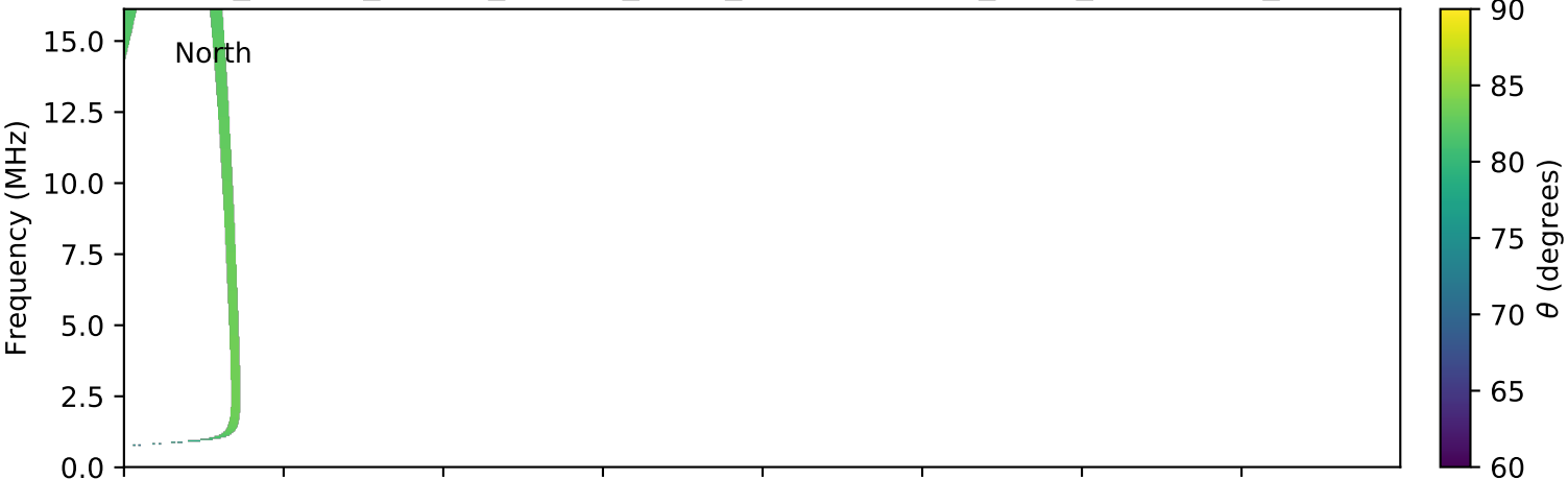
expres_cassini_jupiter_europa_isaac_lossc-wid1deg_3kev_20011015_v01.cdf
