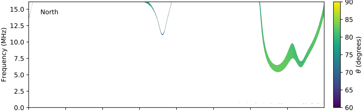
expres_cassini_jupiter_europa_isaac_lossc-wid1deg_3kev_20011014_v01.cdf
