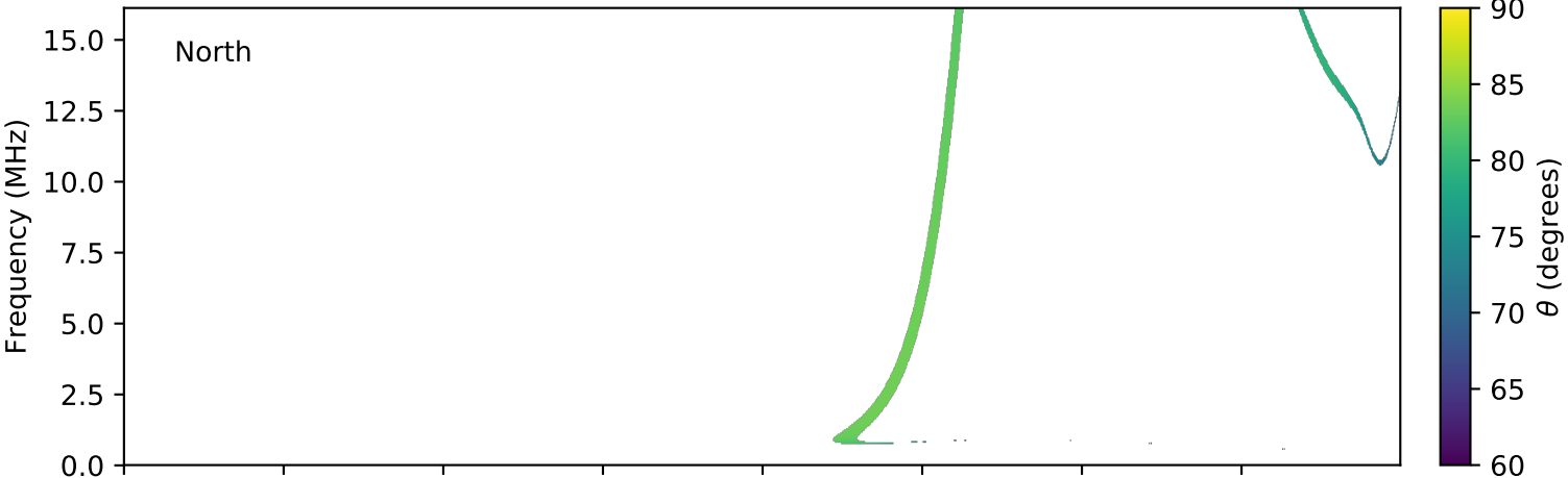
expres_cassini_jupiter_europa_isaac_lossc-wid1deg_3kev_20011013_v01.cdf
