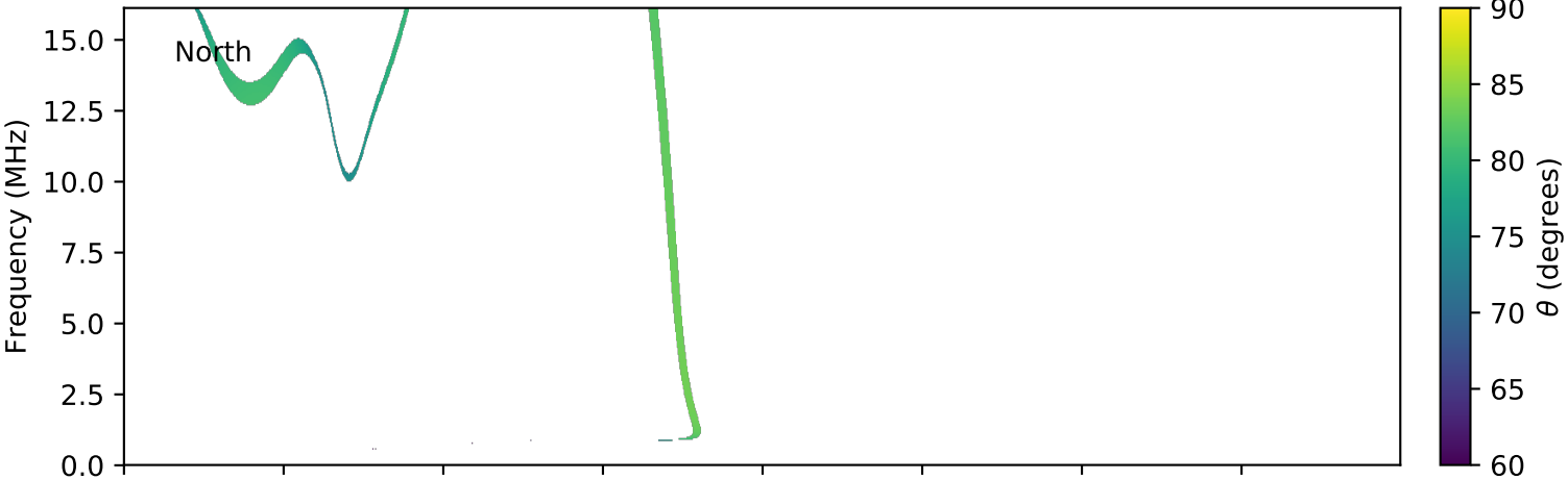
expres_cassini_jupiter_europa_isaac_lossc-wid1deg_3kev_20011011_v01.cdf
