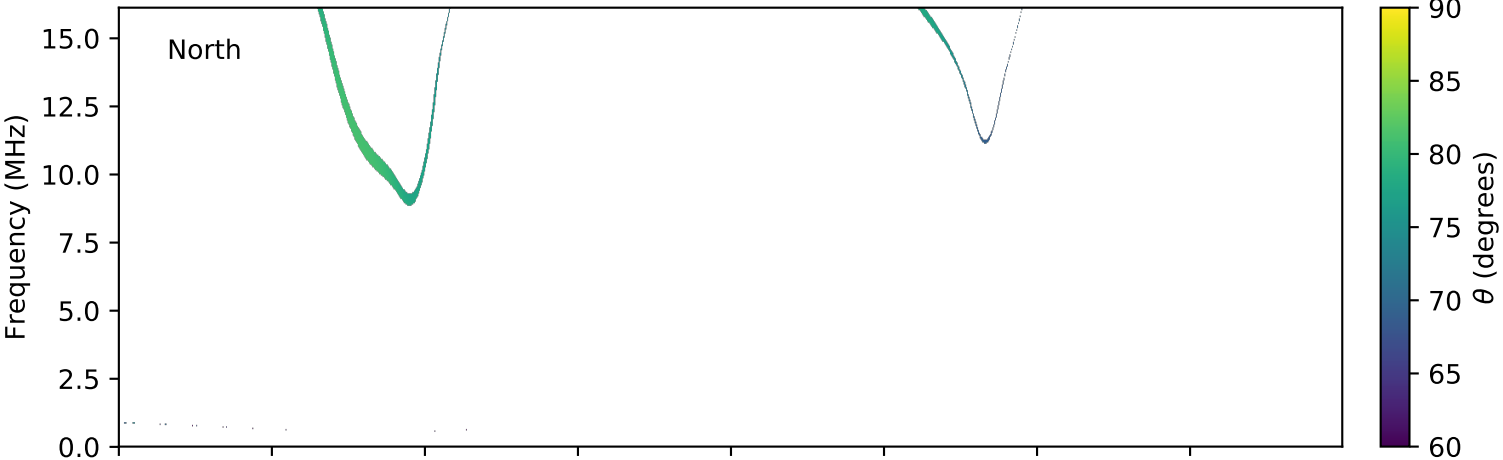
expres_cassini_jupiter_europa_isaac_lossc-wid1deg_3kev_20011010_v01.cdf
