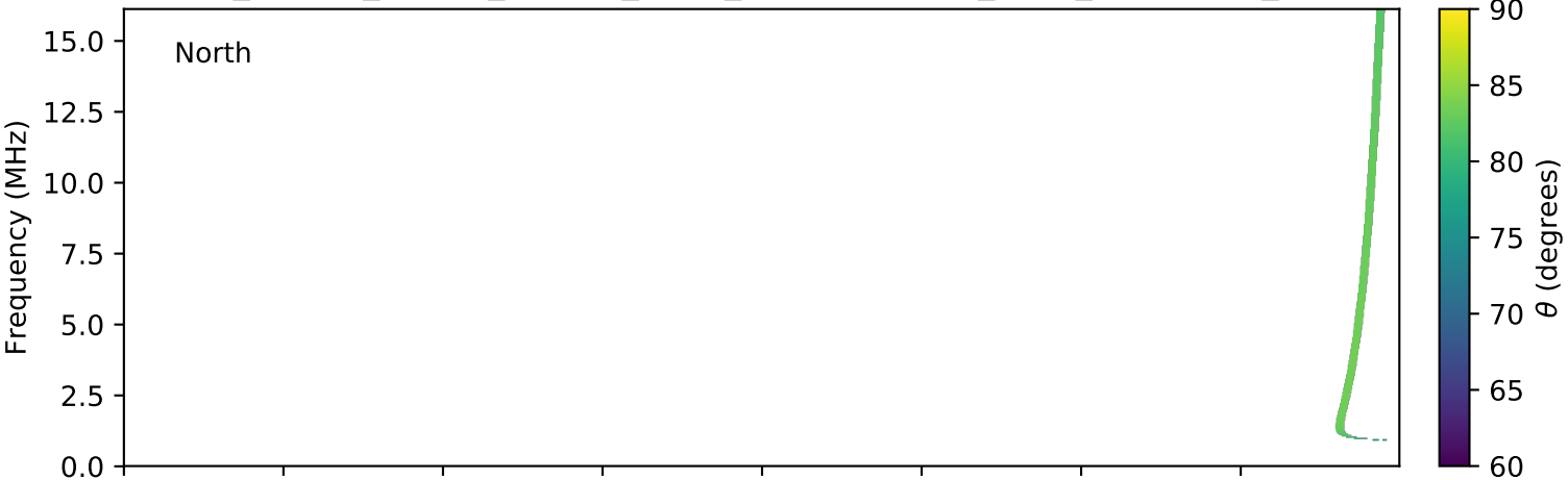
expres_cassini_jupiter_europa_isaac_lossc-wid1deg_3kev_20011009_v01.cdf
