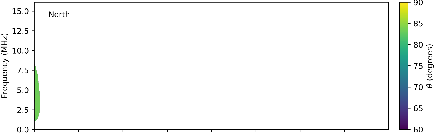
expres_cassini_jupiter_europa_isaac_lossc-wid1deg_3kev_20011008_v01.cdf
