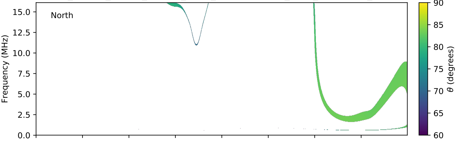
expres_cassini_jupiter_europa_isaac_lossc-wid1deg_3kev_20011007_v01.cdf
