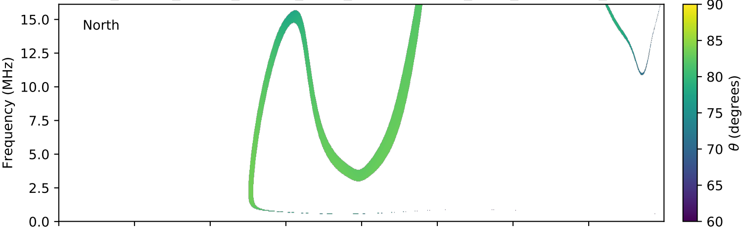
expres_cassini_jupiter_europa_isaac_lossc-wid1deg_3kev_20011006_v01.cdf
