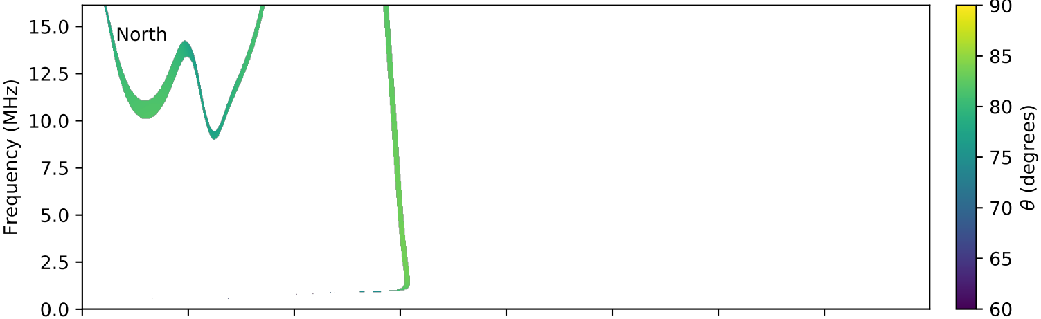
expres_cassini_jupiter_europa_isaac_lossc-wid1deg_3kev_20011004_v01.cdf
