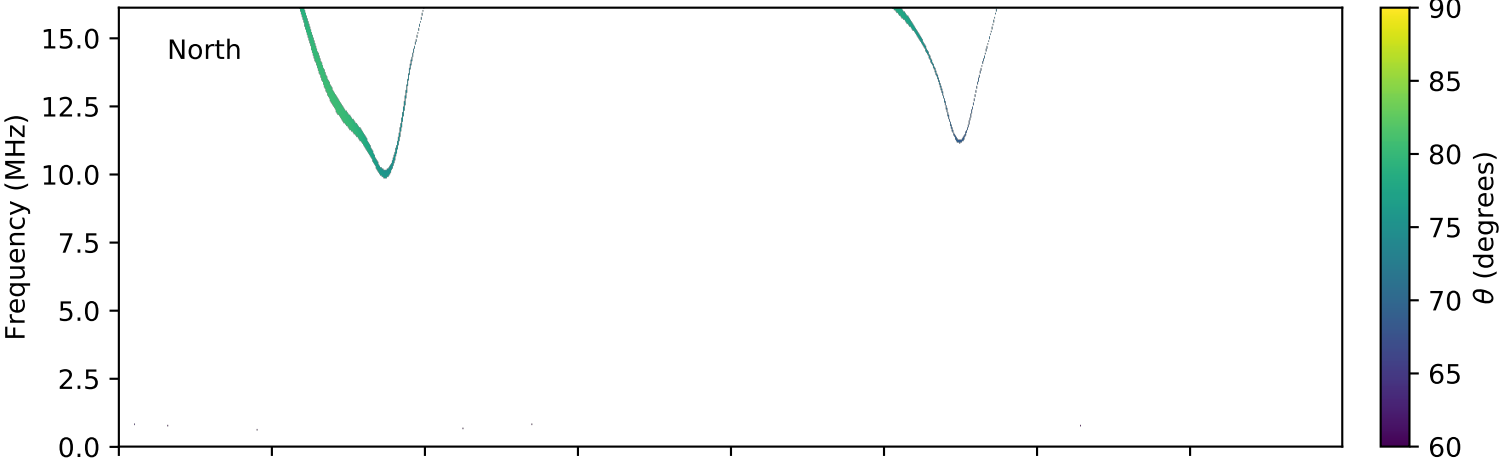
expres_cassini_jupiter_europa_isaac_lossc-wid1deg_3kev_20011003_v01.cdf
