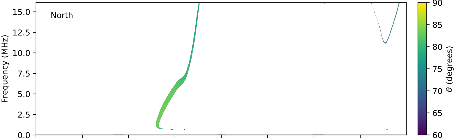
expres_cassini_jupiter_io_isaac_lossc-wid1deg_3kev_20010927_v01.cdf
