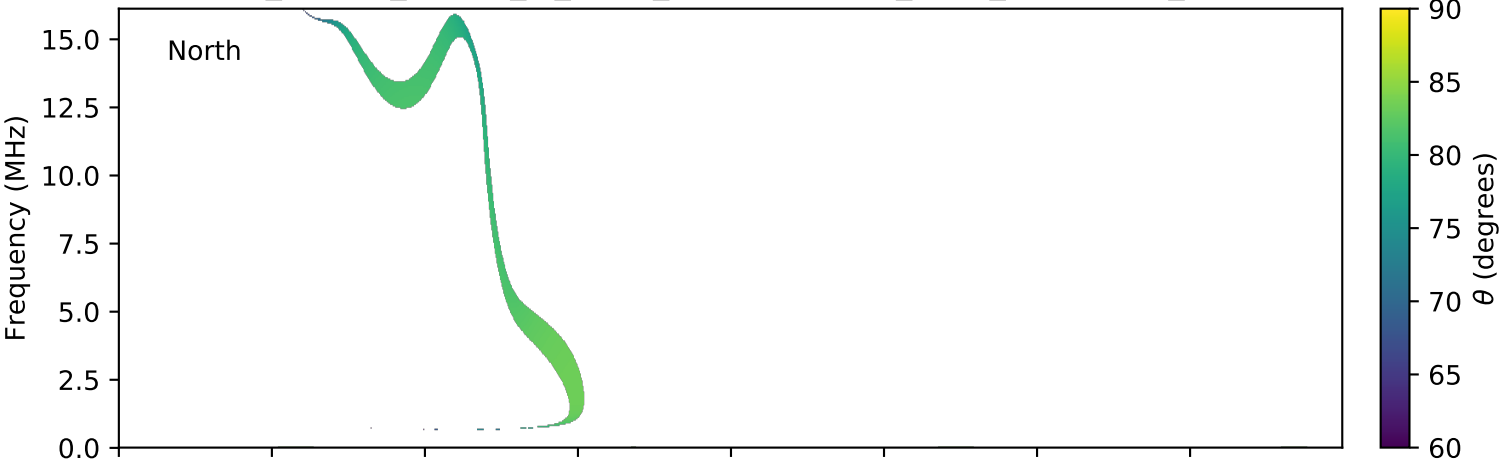
expres_cassini_jupiter_io_isaac_lossc-wid1deg_3kev_20010926_v01.cdf
