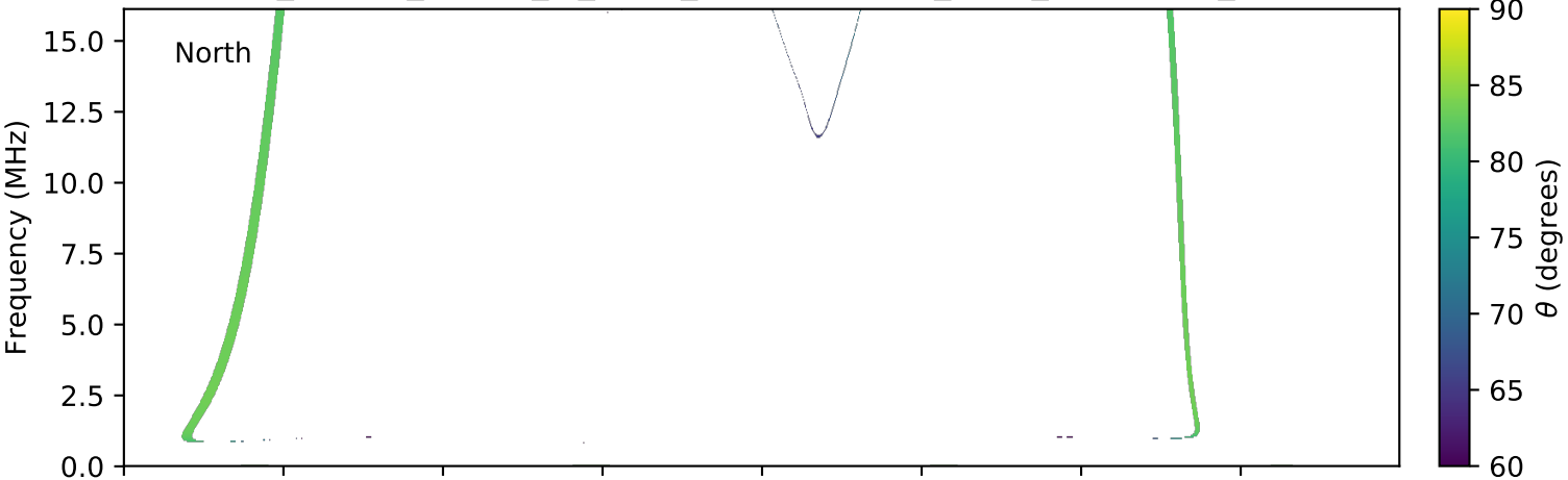
expres_cassini_jupiter_io_isaac_lossc-wid1deg_3kev_20010922_v01.cdf
