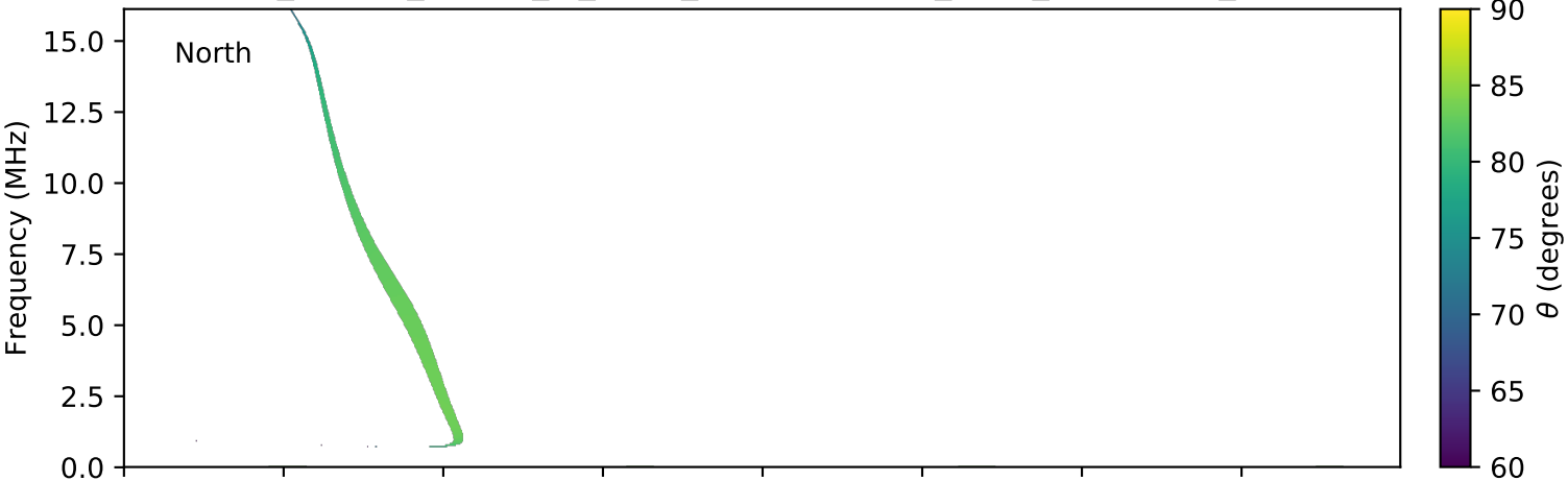
expres_cassini_jupiter_io_isaac_lossc-wid1deg_3kev_20010919_v01.cdf
