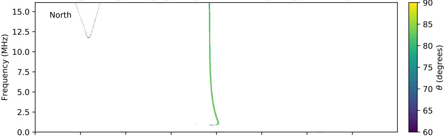
expres_cassini_jupiter_io_isaac_lossc-wid1deg_3kev_20010917_v01.cdf
