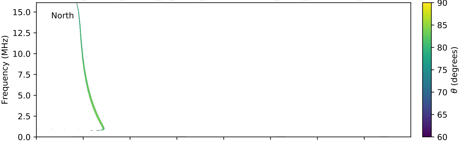
expres_cassini_jupiter_io_isaac_lossc-wid1deg_3kev_20010912_v01.cdf
