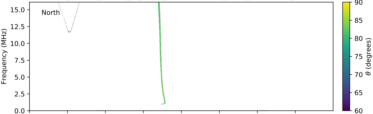
expres_cassini_jupiter_io_isaac_lossc-wid1deg_3kev_20010910_v01.cdf
