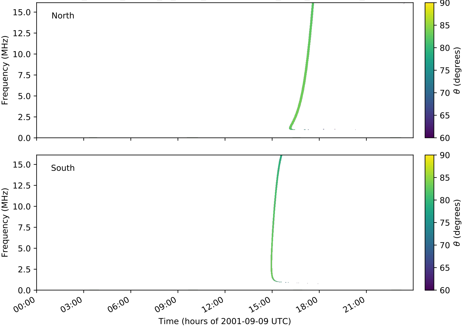
expres_cassini_jupiter_io_isaac_lossc-wid1deg_3kev_20010909_v01.cdf
