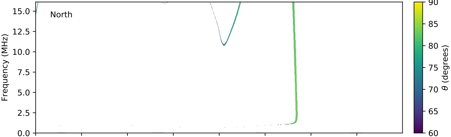
expres_cassini_jupiter_io_isaac_lossc-wid1deg_3kev_20010908_v01.cdf
