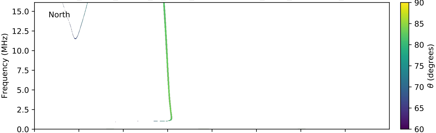
expres_cassini_jupiter_io_isaac_lossc-wid1deg_3kev_20010903_v01.cdf
