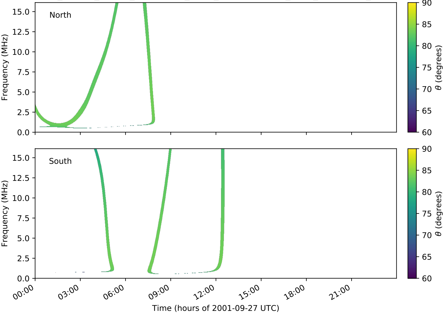
expres_cassini_jupiter_ganymede_isaac_lossc-wid1deg_3kev_20010927_v01.cdf
