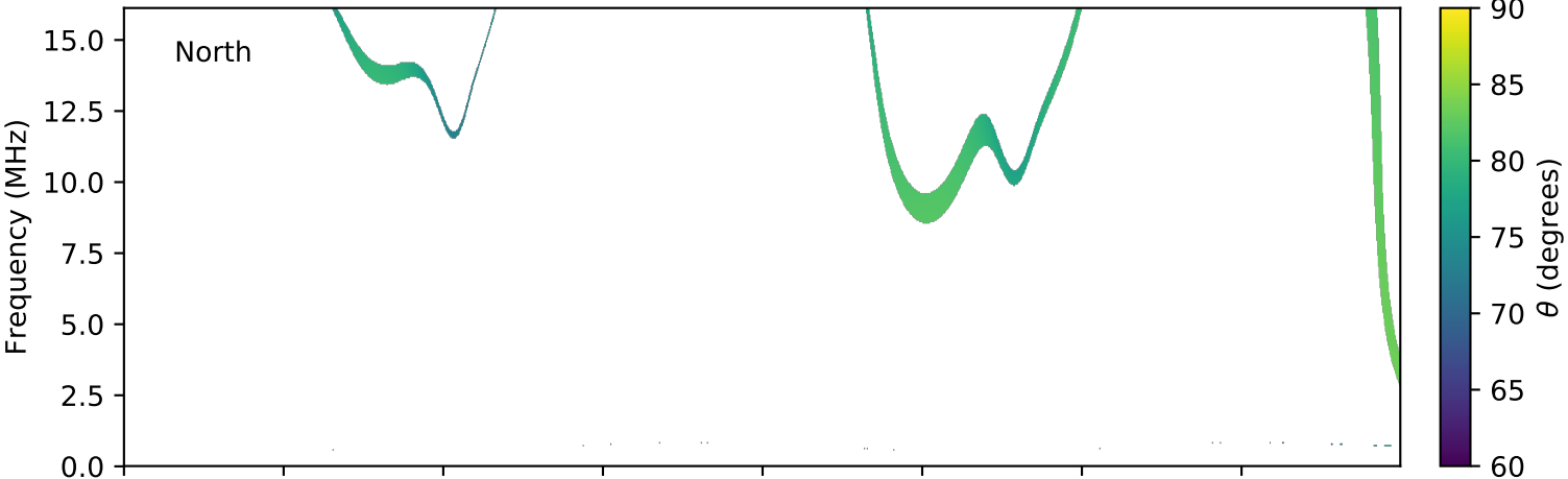
expres_cassini_jupiter_ganymede_isaac_lossc-wid1deg_3kev_20010926_v01.cdf
