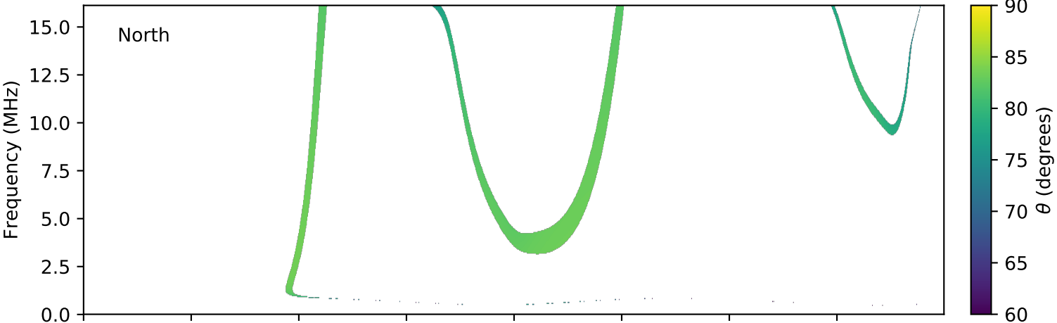
expres_cassini_jupiter_ganymede_isaac_lossc-wid1deg_3kev_20010924_v01.cdf
