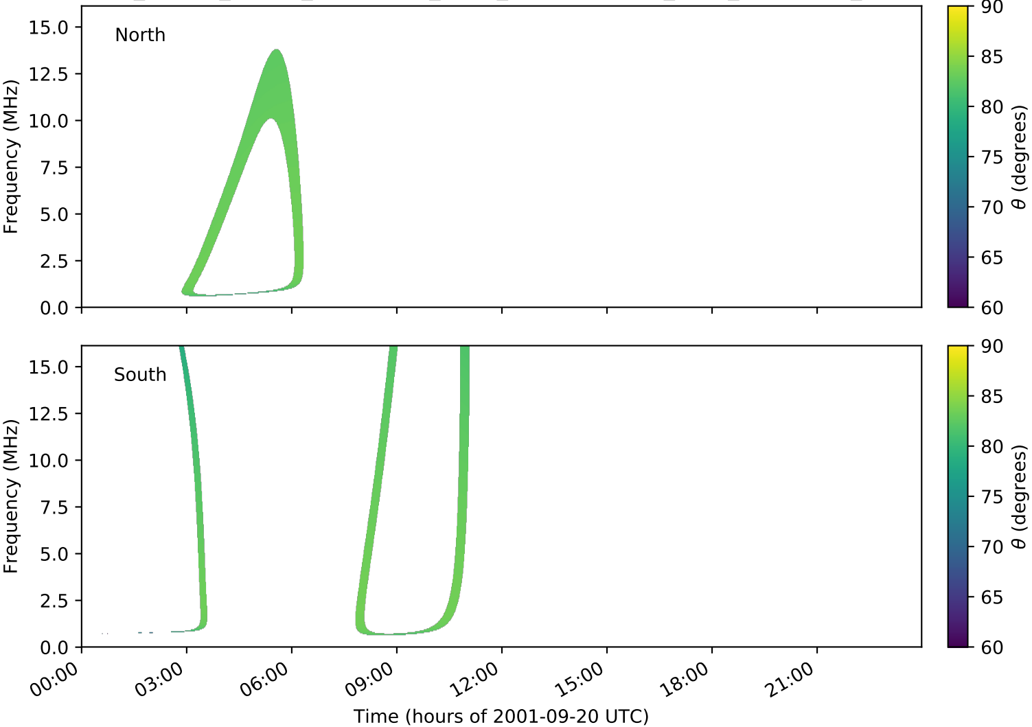
expres_cassini_jupiter_ganymede_isaac_lossc-wid1deg_3kev_20010920_v01.cdf
