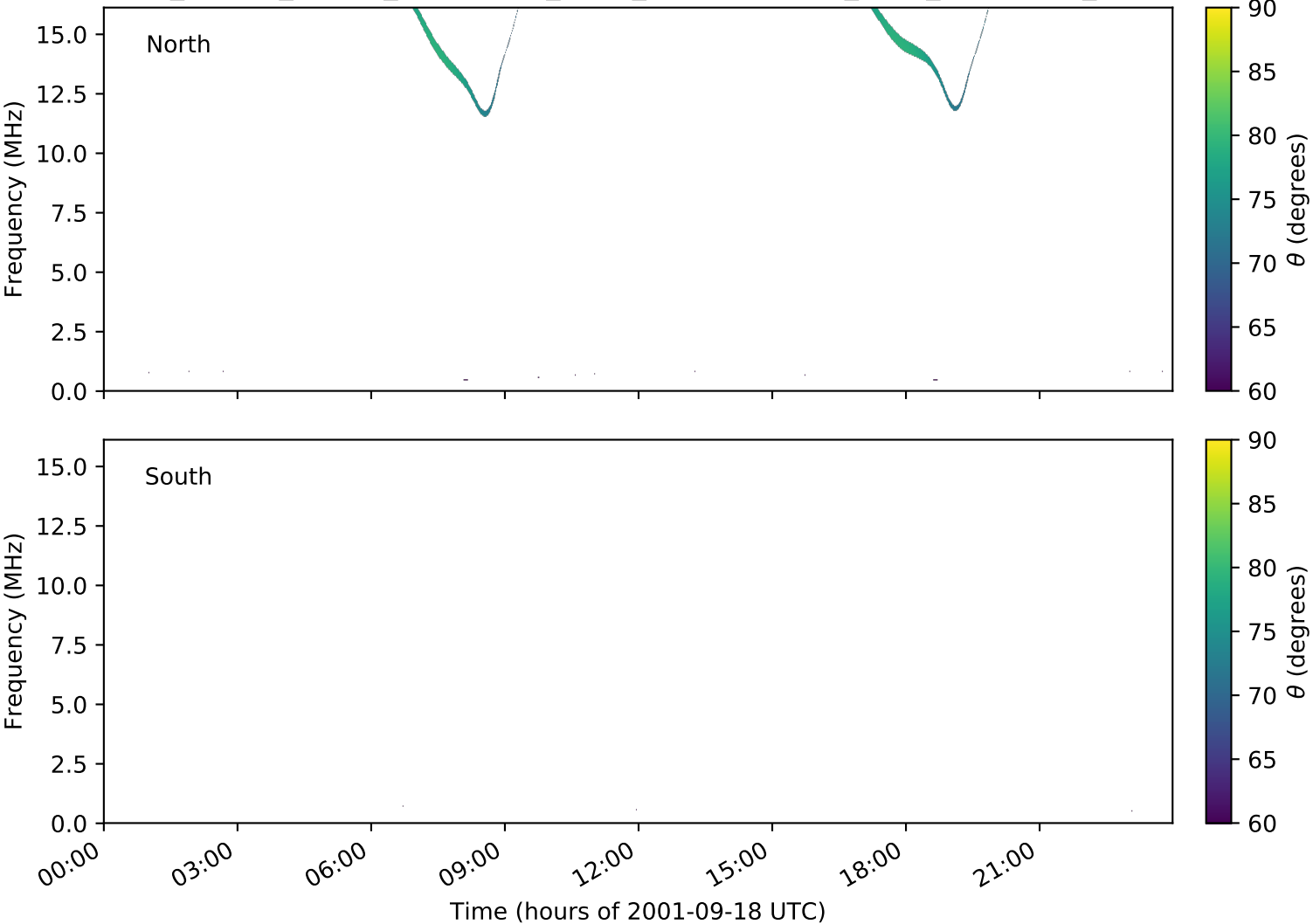
expres_cassini_jupiter_ganymede_isaac_lossc-wid1deg_3kev_20010918_v01.cdf
