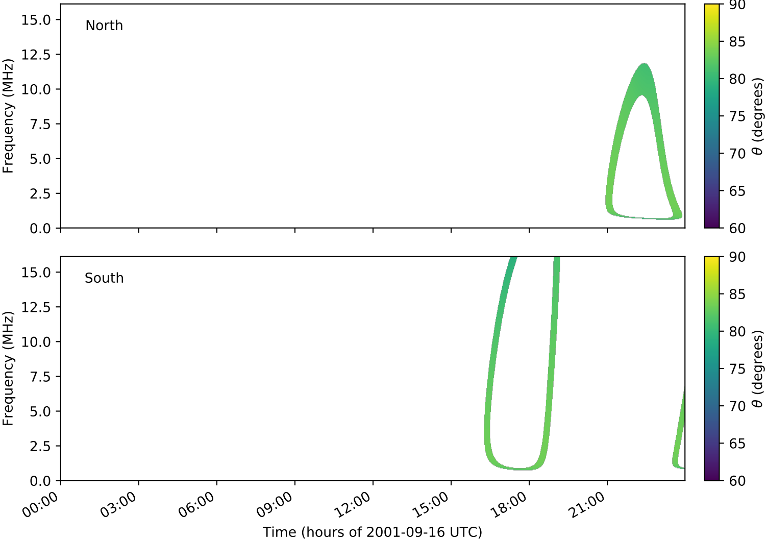
expres_cassini_jupiter_ganymede_isaac_lossc-wid1deg_3kev_20010916_v01.cdf
