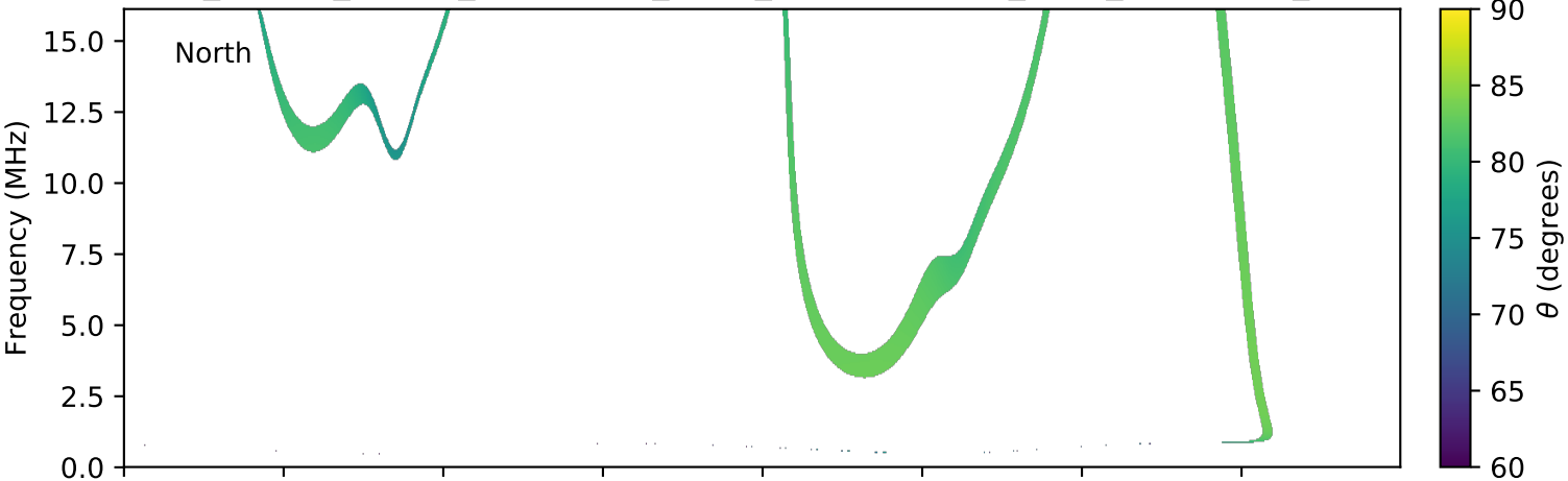
expres_cassini_jupiter_ganymede_isaac_lossc-wid1deg_3kev_20010912_v01.cdf
