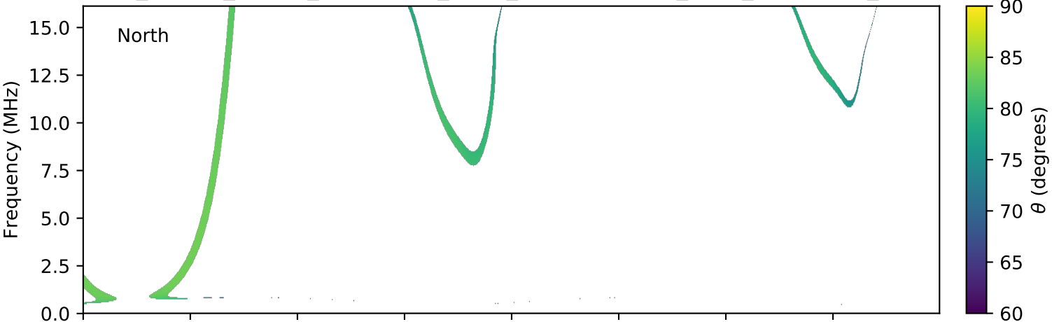
expres_cassini_jupiter_ganymede_isaac_lossc-wid1deg_3kev_20010910_v01.cdf
