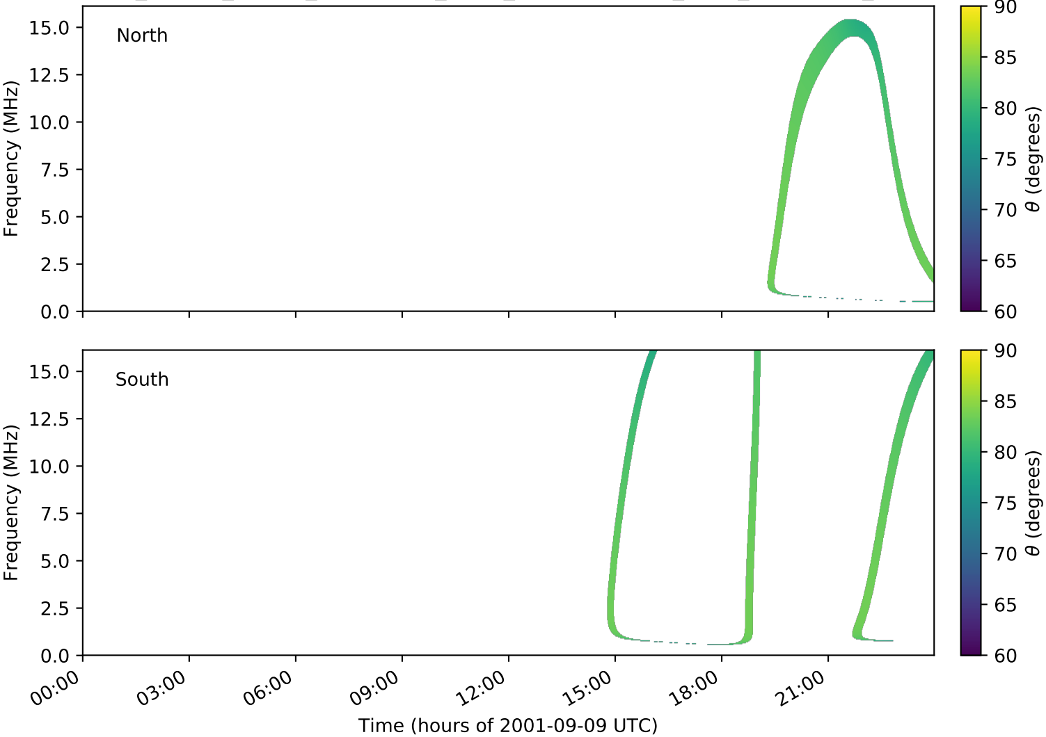
expres_cassini_jupiter_ganymede_isaac_lossc-wid1deg_3kev_20010909_v01.cdf
