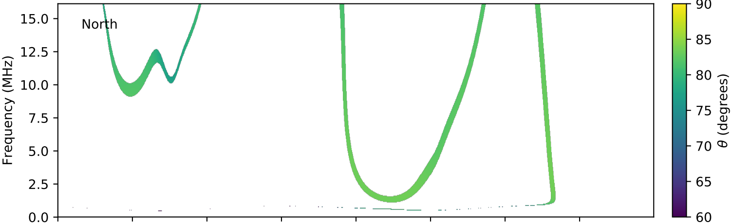
expres_cassini_jupiter_ganymede_isaac_lossc-wid1deg_3kev_20010905_v01.cdf
