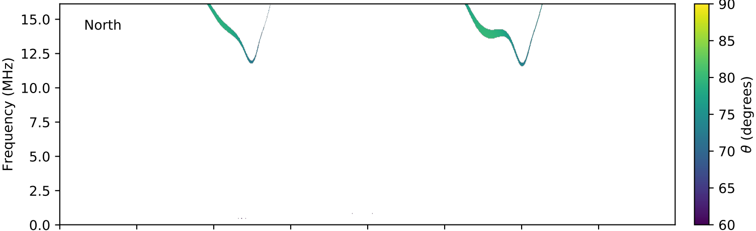
expres_cassini_jupiter_ganymede_isaac_lossc-wid1deg_3kev_20010904_v01.cdf
