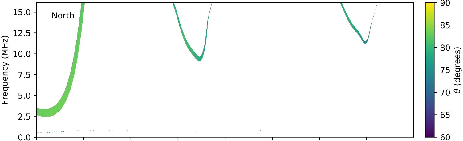
expres_cassini_jupiter_ganymede_isaac_lossc-wid1deg_3kev_20010903_v01.cdf
