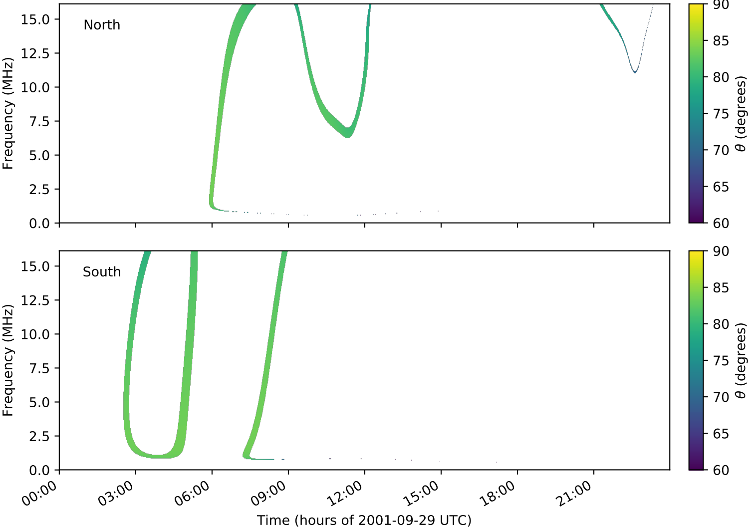
expres_cassini_jupiter_europa_isaac_lossc-wid1deg_3kev_20010929_v01.cdf
