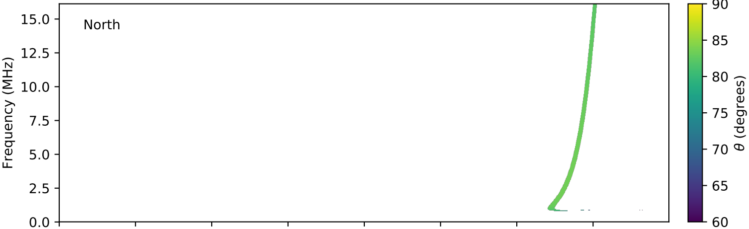
expres_cassini_jupiter_europa_isaac_lossc-wid1deg_3kev_20010925_v01.cdf
