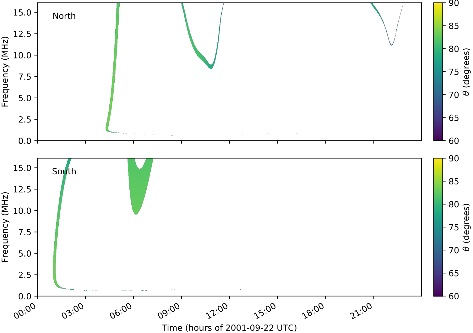
expres_cassini_jupiter_europa_isaac_lossc-wid1deg_3kev_20010922_v01.cdf
