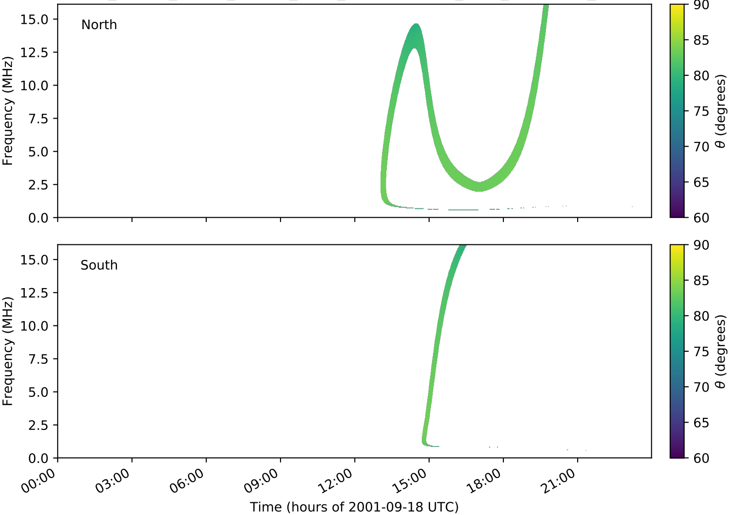
expres_cassini_jupiter_europa_isaac_lossc-wid1deg_3kev_20010918_v01.cdf
