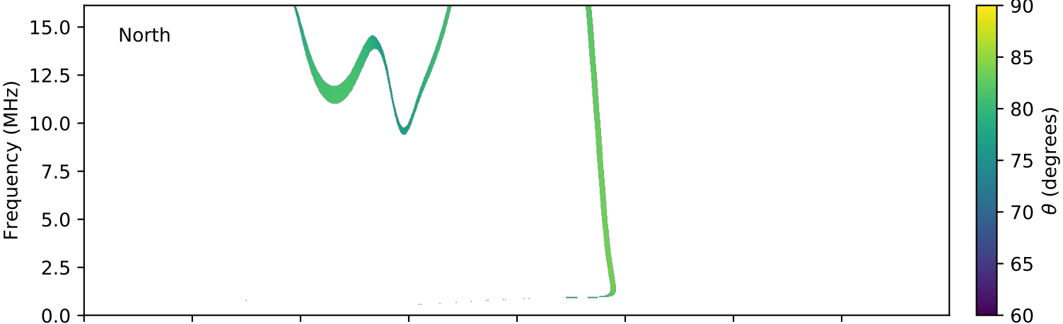
expres_cassini_jupiter_europa_isaac_lossc-wid1deg_3kev_20010916_v01.cdf
