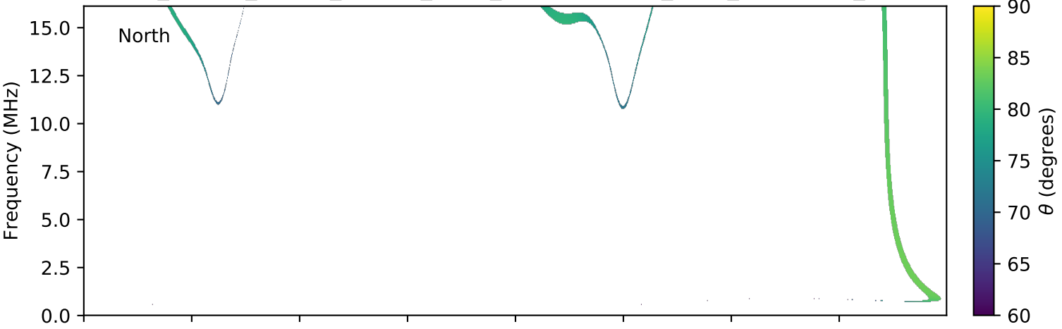
expres_cassini_jupiter_europa_isaac_lossc-wid1deg_3kev_20010912_v01.cdf
