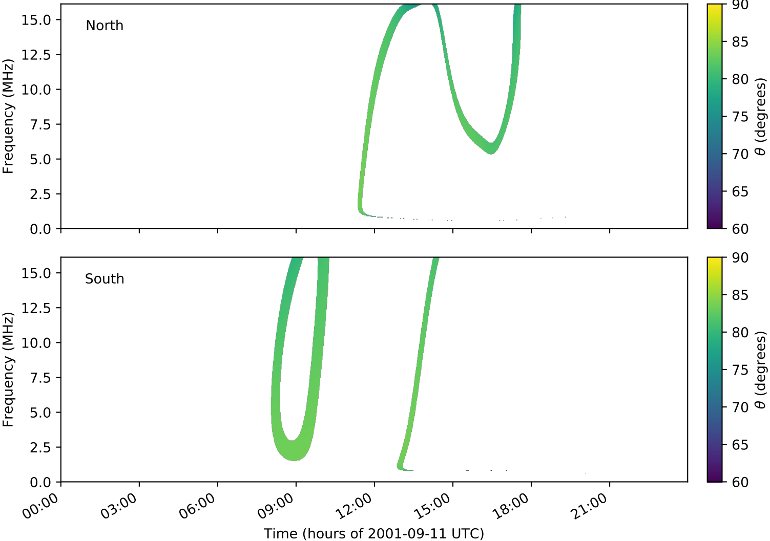
expres_cassini_jupiter_europa_isaac_lossc-wid1deg_3kev_20010911_v01.cdf
