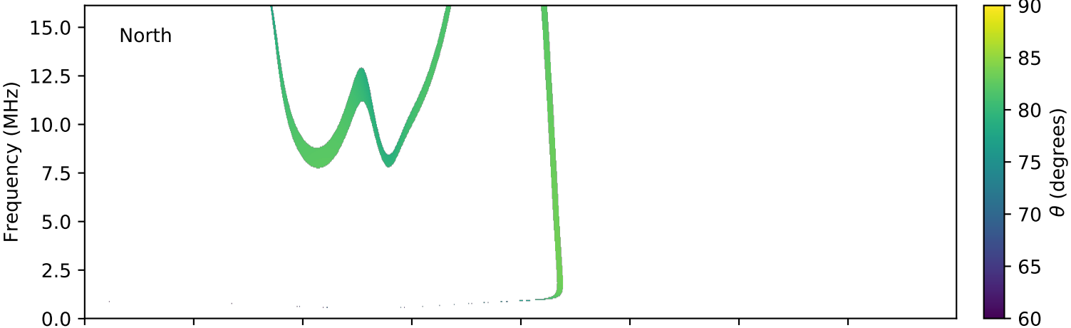
expres_cassini_jupiter_europa_isaac_lossc-wid1deg_3kev_20010909_v01.cdf
