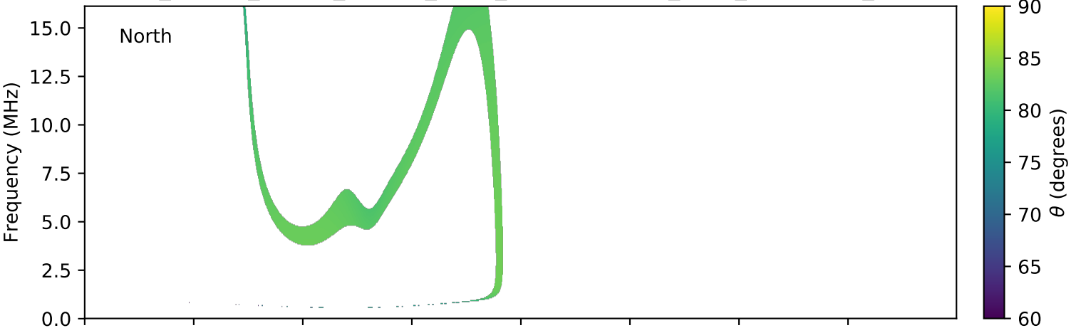
expres_cassini_jupiter_europa_isaac_lossc-wid1deg_3kev_20010902_v01.cdf
